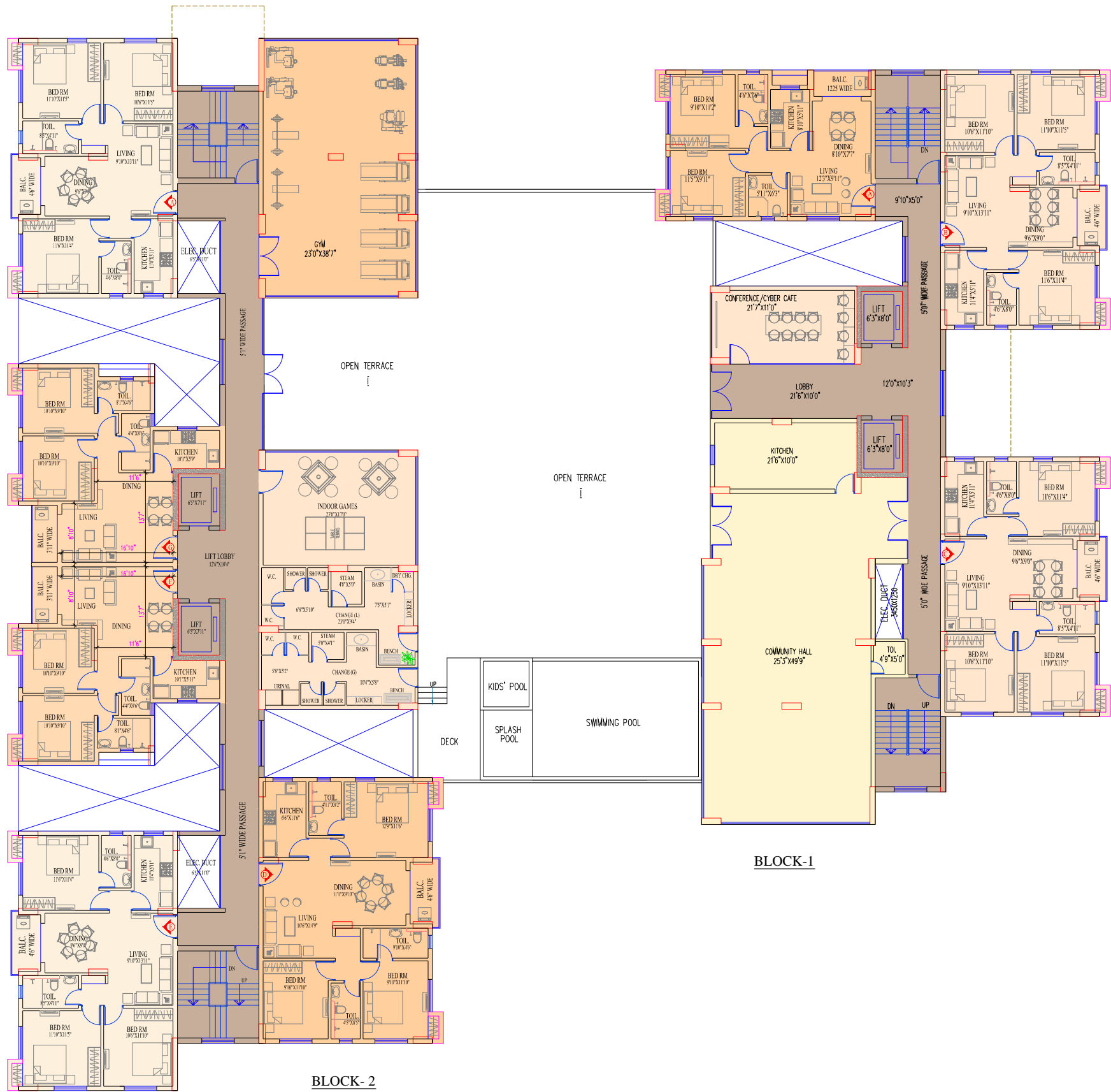
FIRST FLOOR PLAN BLOCK-1 & 2 SCALE * 1:100
